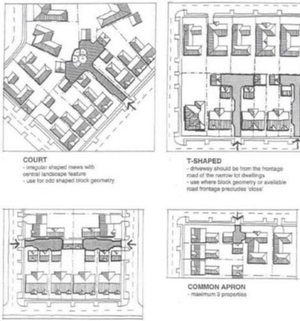
Figure E17.32: Shared Driveway Principles
