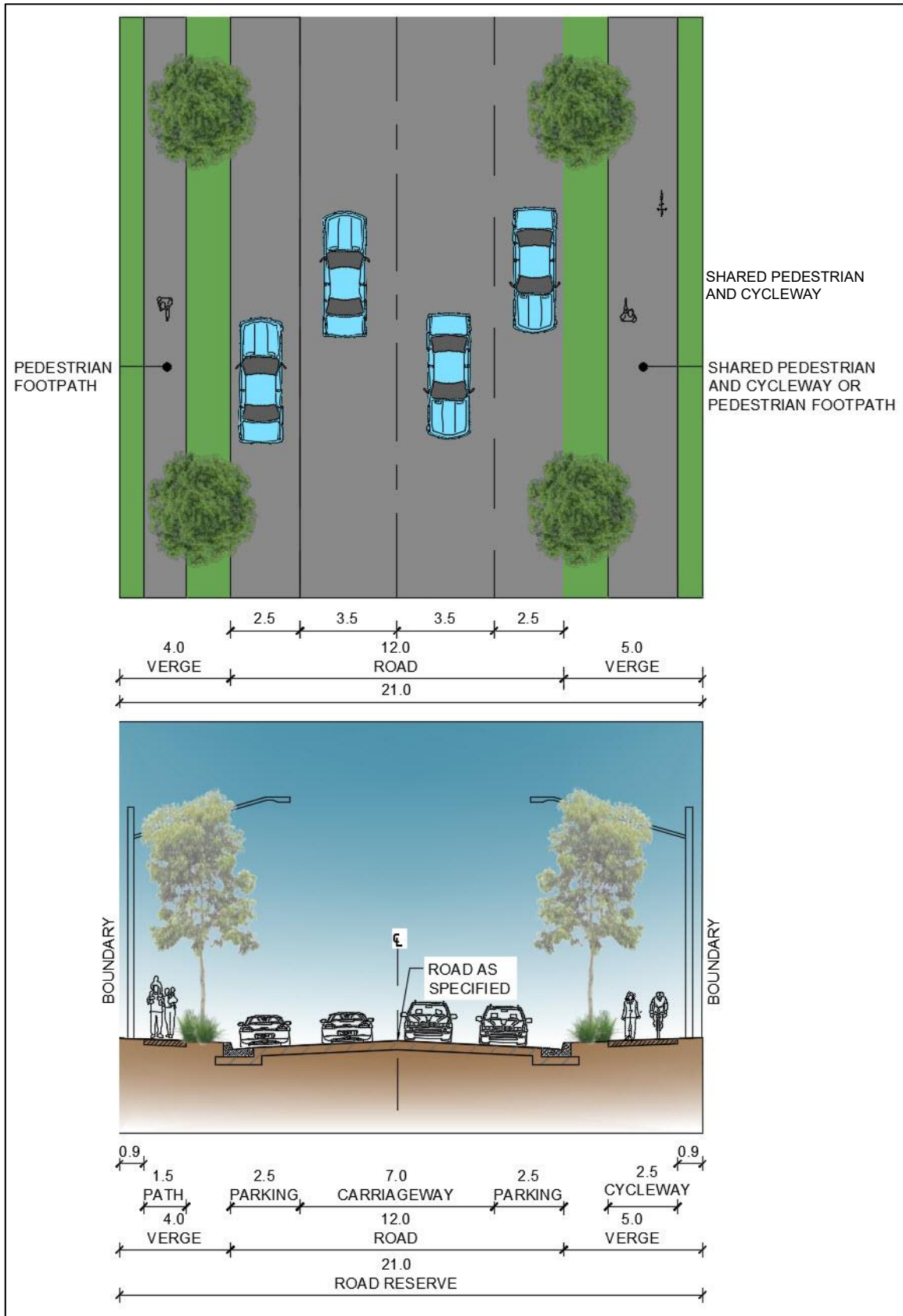
Figure E17.11: Typical street cross section – Major Local Road
