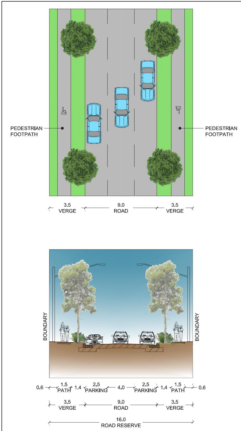
Figure E17.1: Typical street cross section – Minor Local Road
