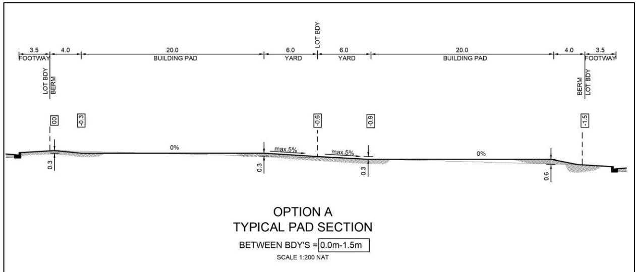
Figure E17.22: Typical Grading Solutions
